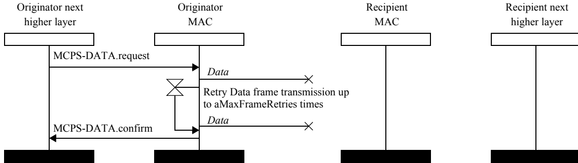
Figure 6-41—Lost Data frame message sequence
