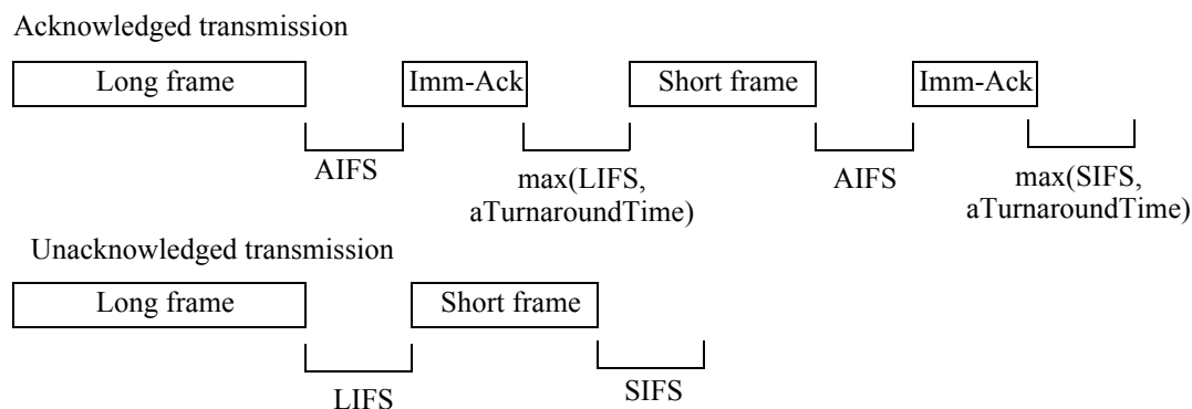
Figure 6-4—IFS usage
