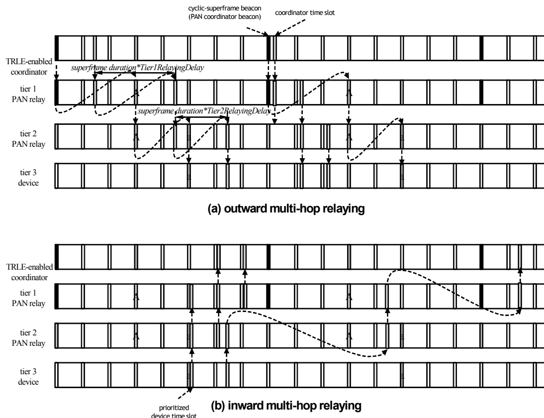
Figure F.5—Synchronous multi-hop frame relaying
