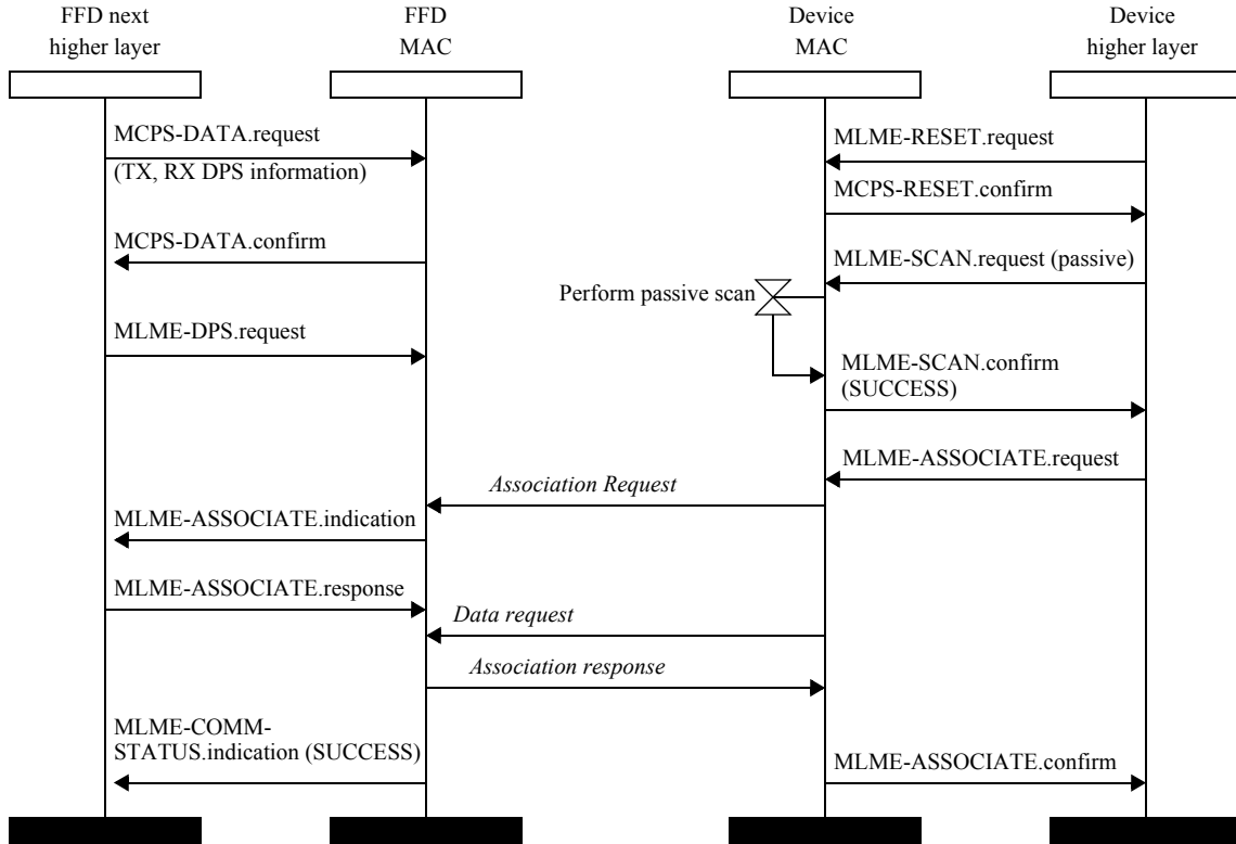
Figure 6-22—Association message sequence chart
