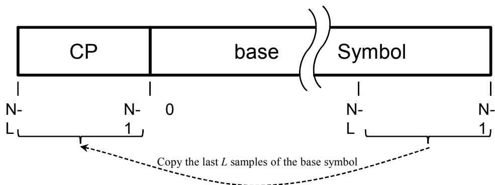
Figure 21-13—Cyclic prefix (CP)
