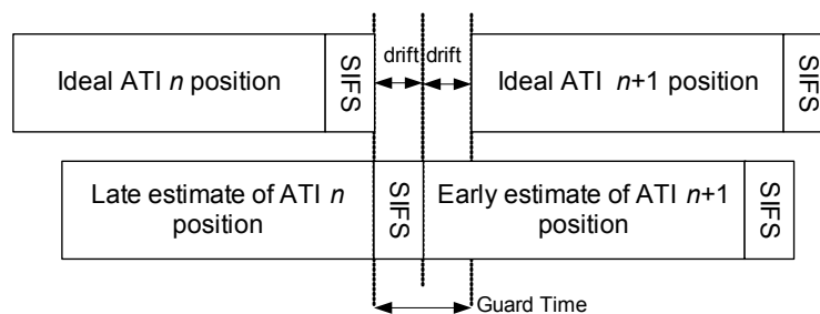
Figure 6-36—Guard time
