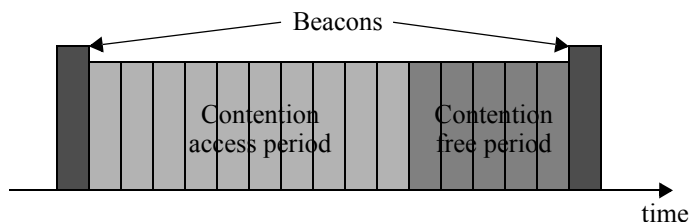
Figure 5-6—Structure of the active periods with GTSs
