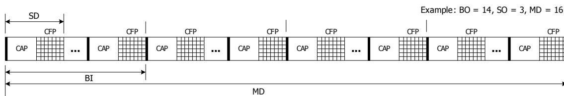
Figure 6-50—Example of DSME multi-superframe structure (MO>BO)
