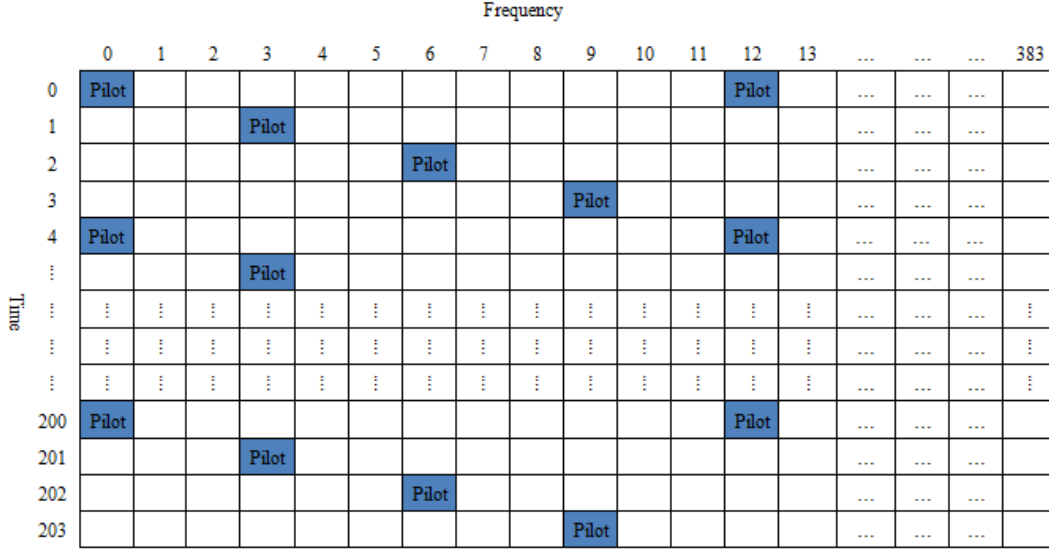
Figure 27-11—Pattern of pilot subcarriers allocated in TVWS-NB-OFDM symbol
