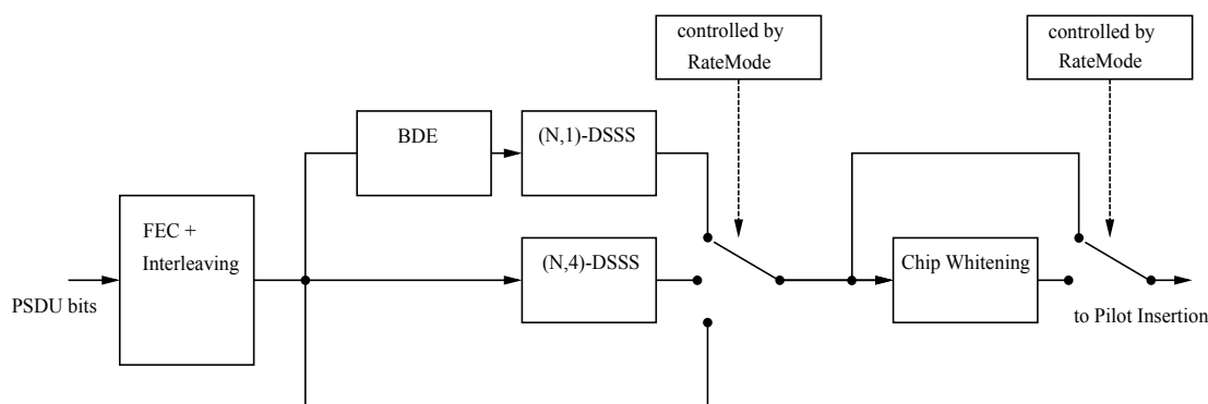
Figure 22-8—PSDU processing for DSSS
