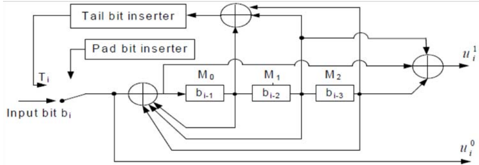
Figure 20-13—The recursive and systematic code (RSC) encoder
