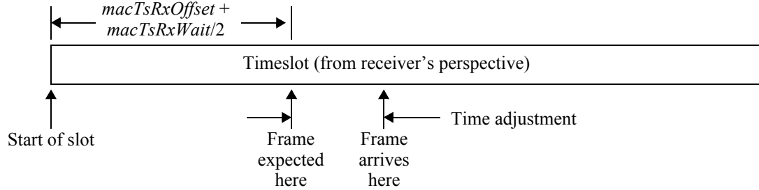
Figure 6-31—Time synchronization
