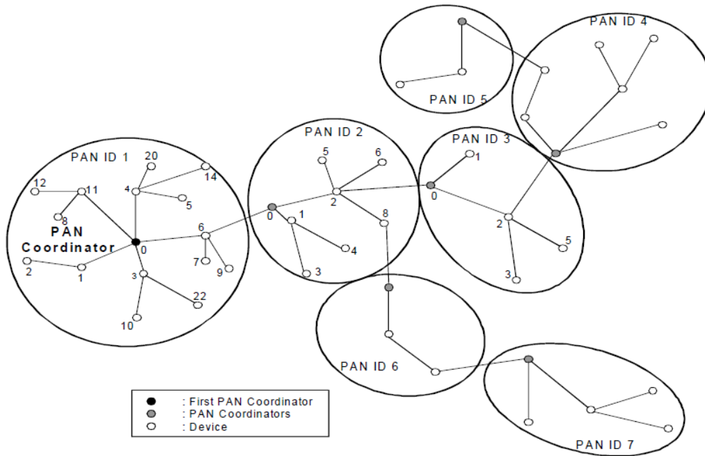
Figure 5-2—Cluster tree network
