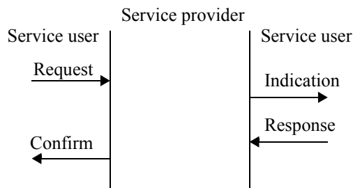
Figure 5-10—Service primitives
