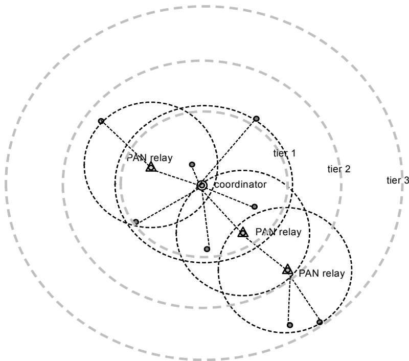
Figure F.3—Hierarchy of relaying in the TRLE-enabled PAN
